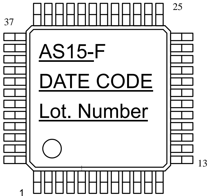
LEAD FREE TQFP48 ( MAKING )
