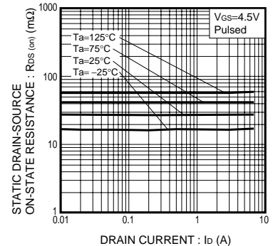
Fig.3 Static Drain-Source On-State Resistance vs. Drain Current(II)
