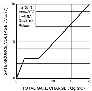
Fig.8 Dynamic Input Characteristics
