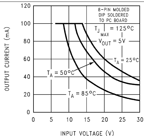
Figure 27. LP2951-N Maximum Rated Output Current
