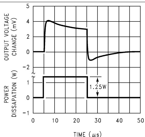
Figure 29. Thermal Response
